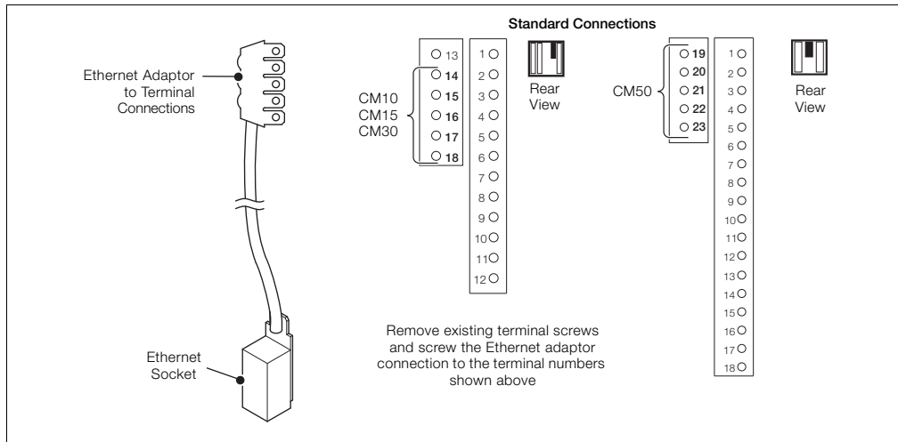
Fig. 7.1 Ethernet Connections
