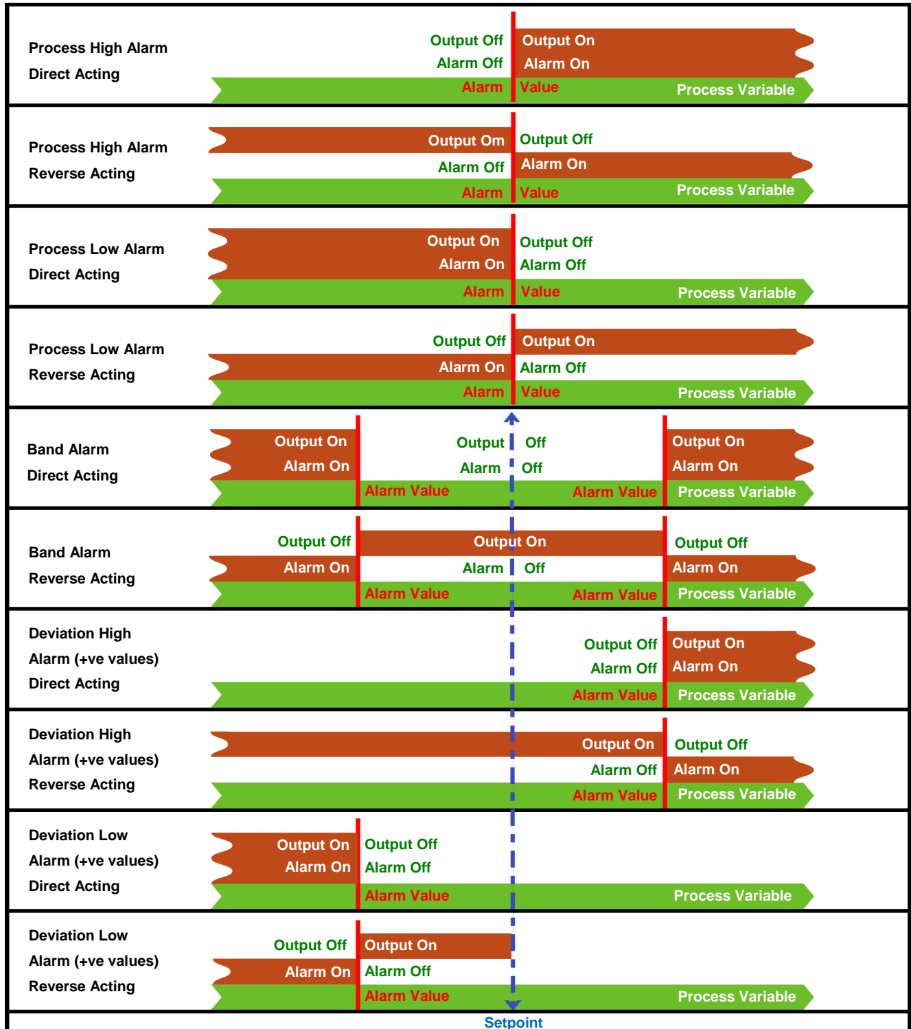
Figure 64. Alarm Operation
