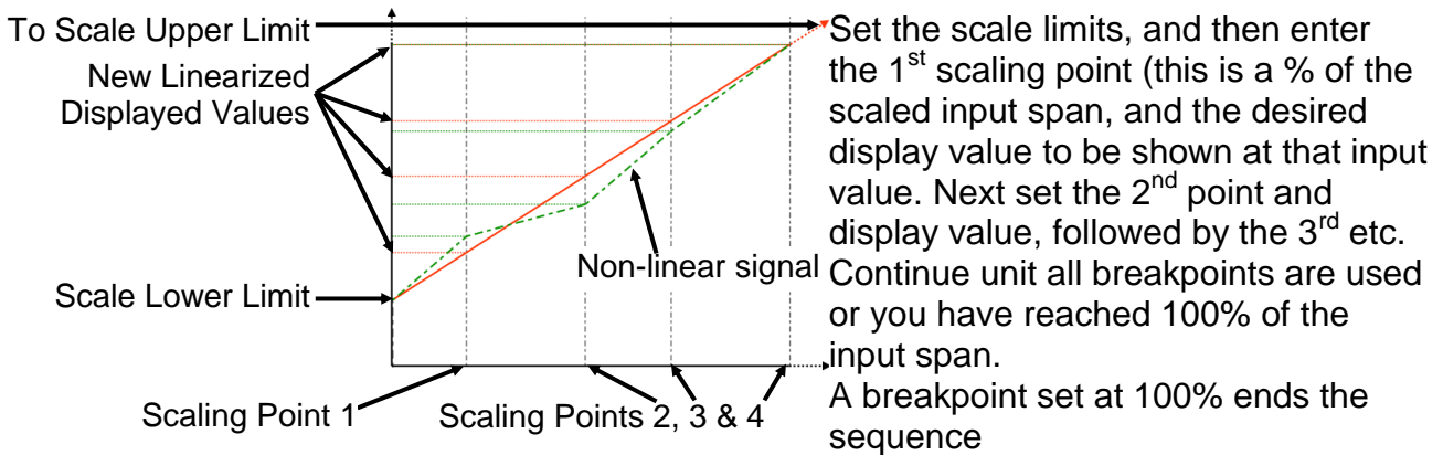
Figure 46. Multi-point Scaling
