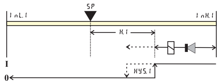
② Operating principle relative alarm L.I = OFF
