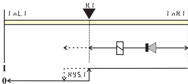
① Operating principle absolut alarm L.I = OFF
