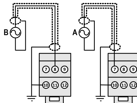
Single core screened cable
