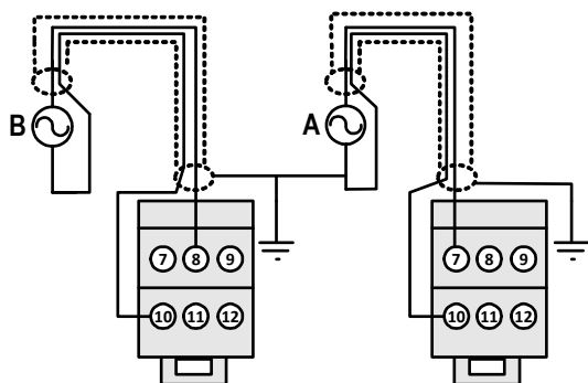
Screened cable
