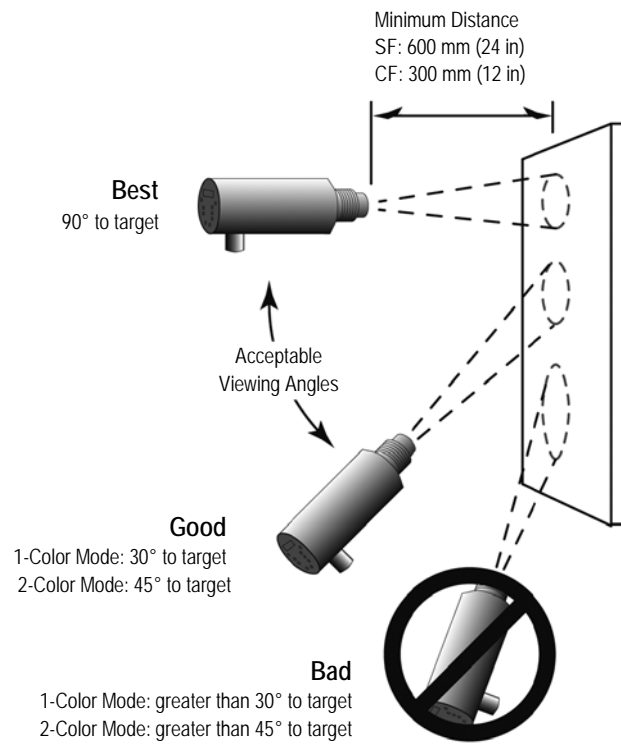
Figure 9: Acceptable Sensor Viewing Angles
