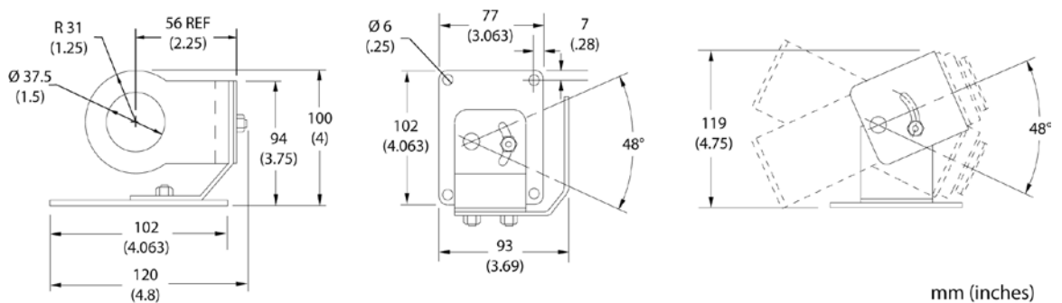
Figure 5: Adjustable Bracket
