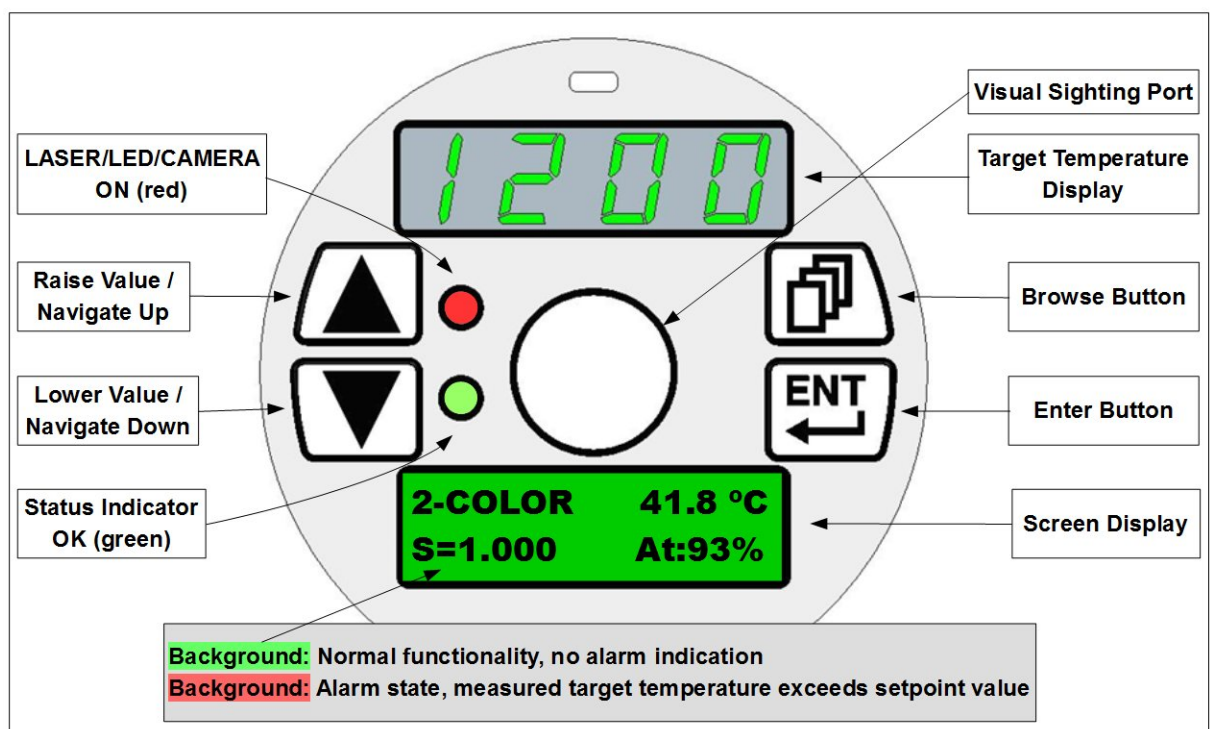
Figure 19: Control Panel
