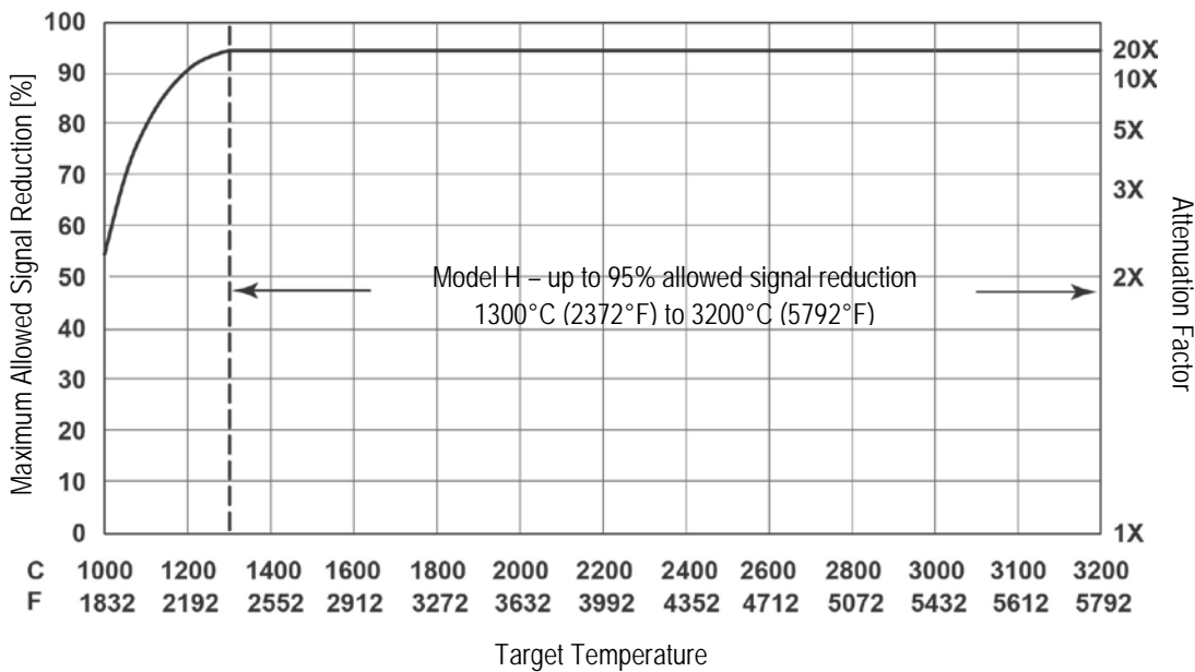
Figure 34: Model H Percentage of Allowed Signal Reduction
