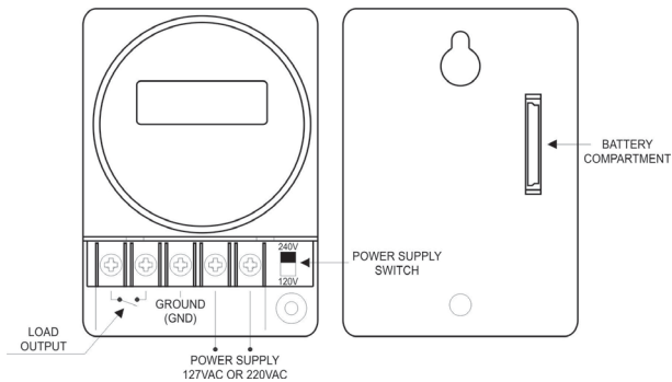
Fig. 03 - The front and the back sight of Timer TM-6331
