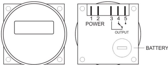
Fig. 02 - The front and the back sight of Timer TM-619
