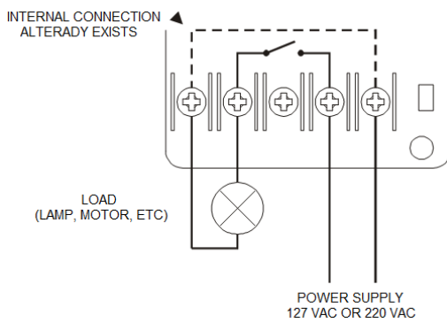
Fig. 07 - TM-6331: Timer Connection
