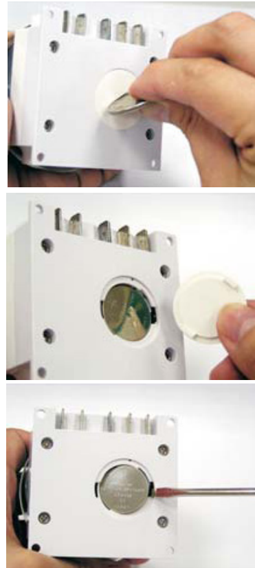
Fig. 05 - Instruction to replace the TM-619's battery
