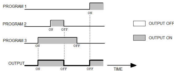
Fig. 01 - Output's Behavior with overlapping programs
