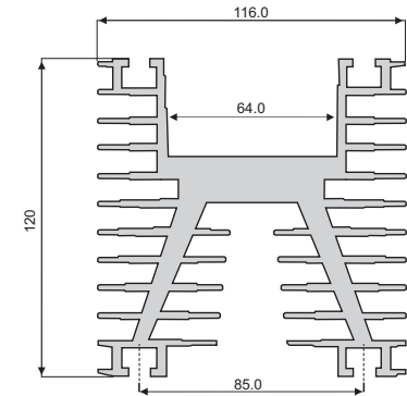
Fig. 5 - Sink ND40 (to 100 mm: R thsa = 0.65 °C / W)
