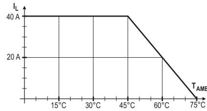
Fig. 3 - SSR2540/4840 + sink ND40-100 mm
