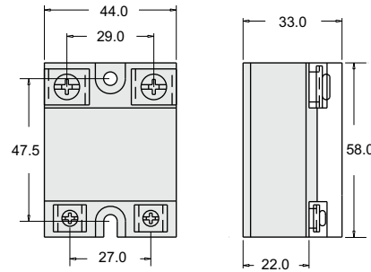
Fig 2 - Dimensions
