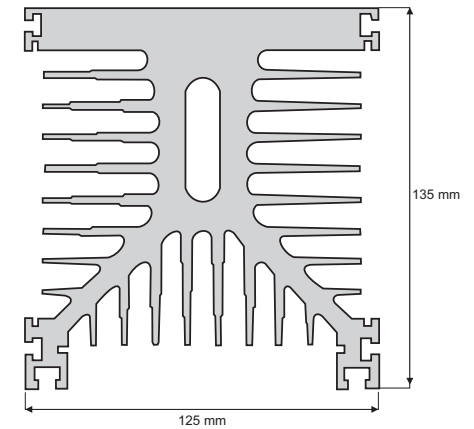
Fig. 6 - Sink NDP3 (to 120 mm: R thsa = 0.52 °C / W)
