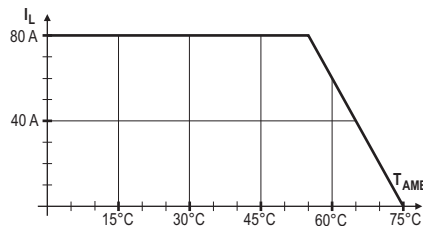
Fig. 4 - SSR4880 + sink NDP3-120 mm + Fun 3 m/s
