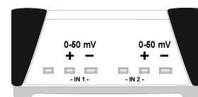
Figure 05 — 0-50 signal connection
