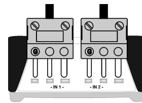
Figure 03 – Pt100 connectors sensors
