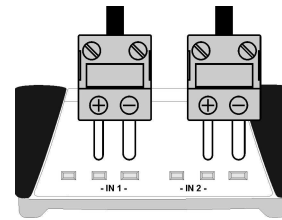
Figure 02 — Thermocouple connection
