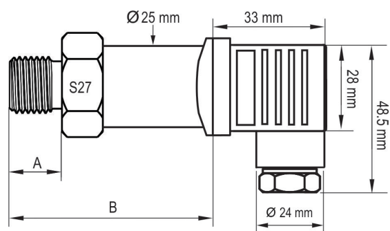
Fig. 5 – Transmitter dimensions
