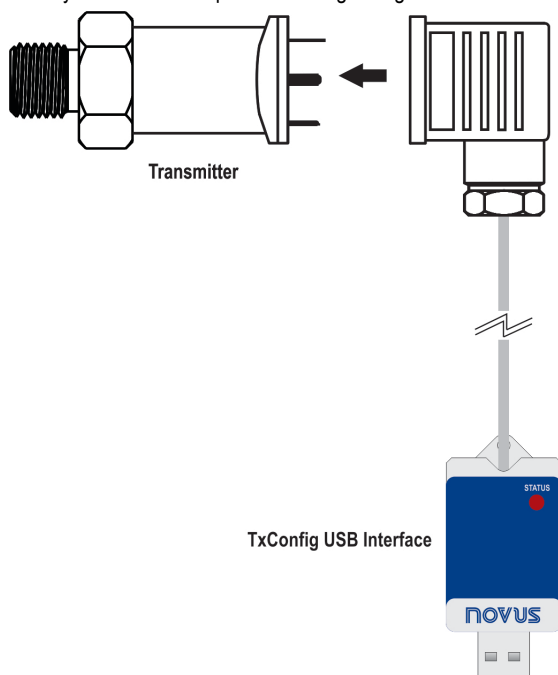
Fig. 3 – Connection of the TxConfig-USB
