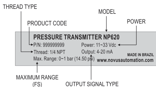
Fig. 1 – Transmitter identification
