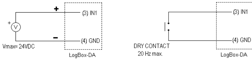
Fig. 10 – Voltage pulse and dry contact channel 1 input
