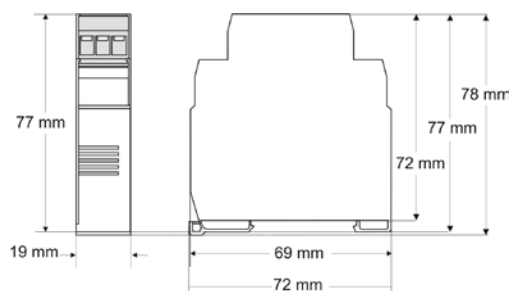
Figure 1 – Dimensions
