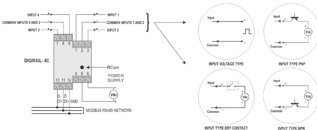
Figure 2 – Electrical Connections
