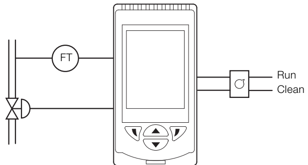
Fig. 8: Remote auto / manual switching
