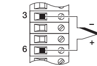
e – Thermocouple
