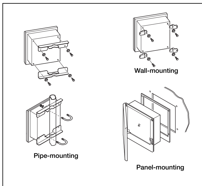
Choice of Mounting Options
