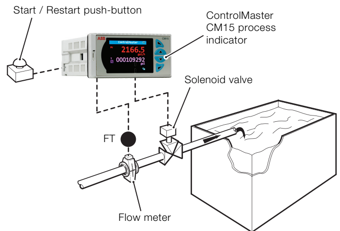
Fig. 1: Batch dispensing process overview
